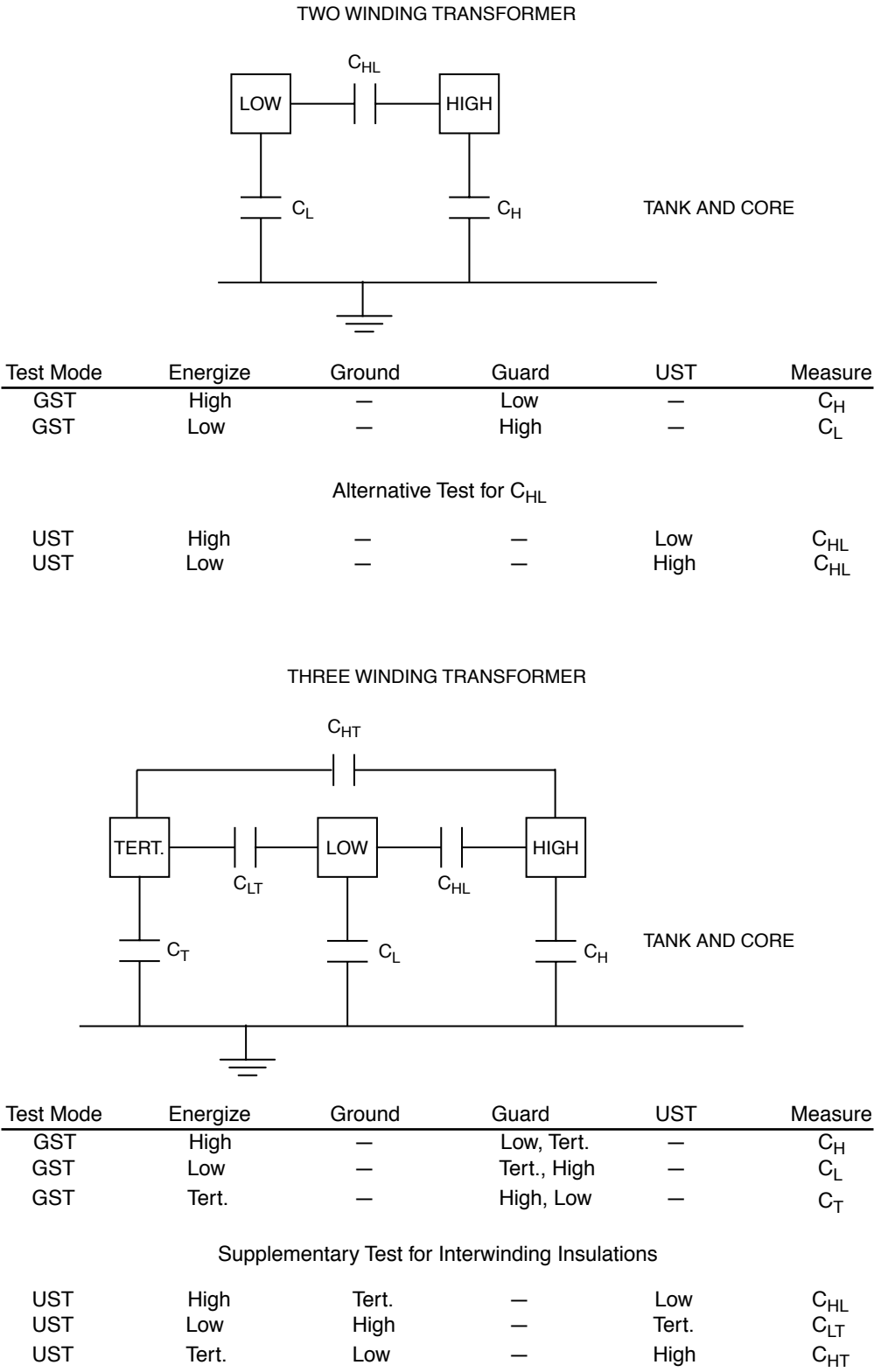
Figure A.2—Test connections for direct measurement of individual component
