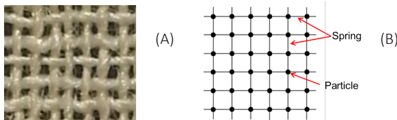
FIGURE 4: PARTICLE MESH PRINCIPLE; (A) PLAIN WEAVE, (B) PARTICLE-SPRING MESH, THE PARTICLES REPRESENT THE YARN INTERSECTIONS
