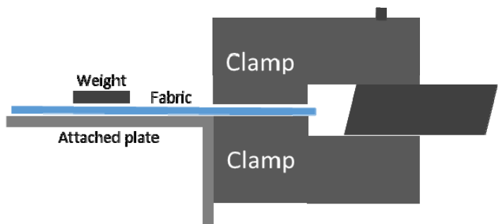
FIGURE 15: OPTITEX MARK 10, ATTACHMENT CONFIGURATION FOR FRICTION MEASUREMENT
