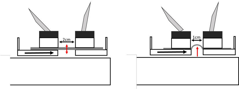
FIGURE 10: SCHEMATIC DIAGRAM OF THE FAB UPWARD BENDING MEASUREMENT
