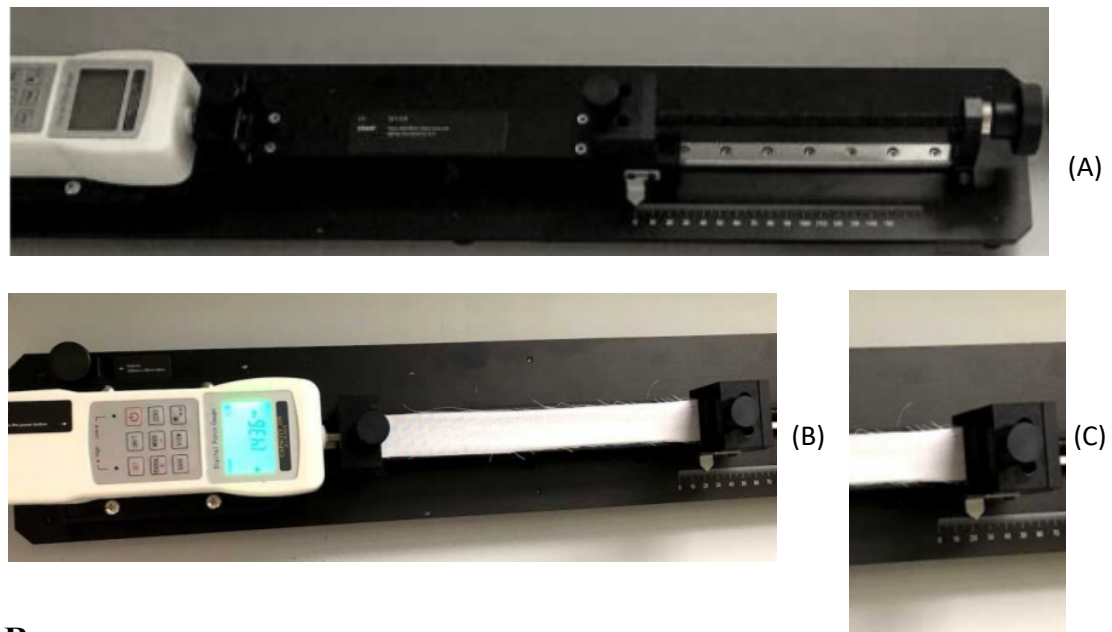
FIGURE 14: TENSILE TESTING
